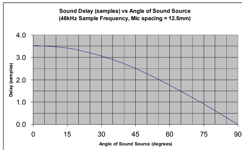
Figure 2 Delay Between Channels vs Angle of Sound Source
