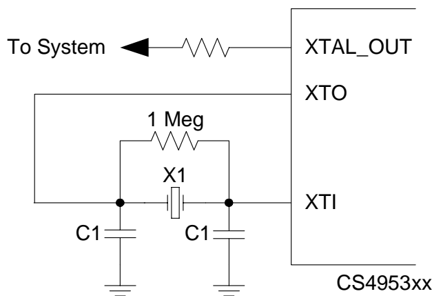
Figure 9-10. Crystal Oscillator Circuit Diagram
