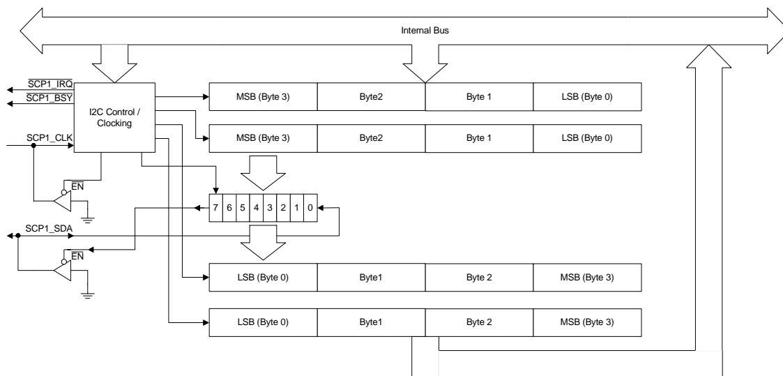
Figure 3-1. Serial Control Port Internal Block Diagram
