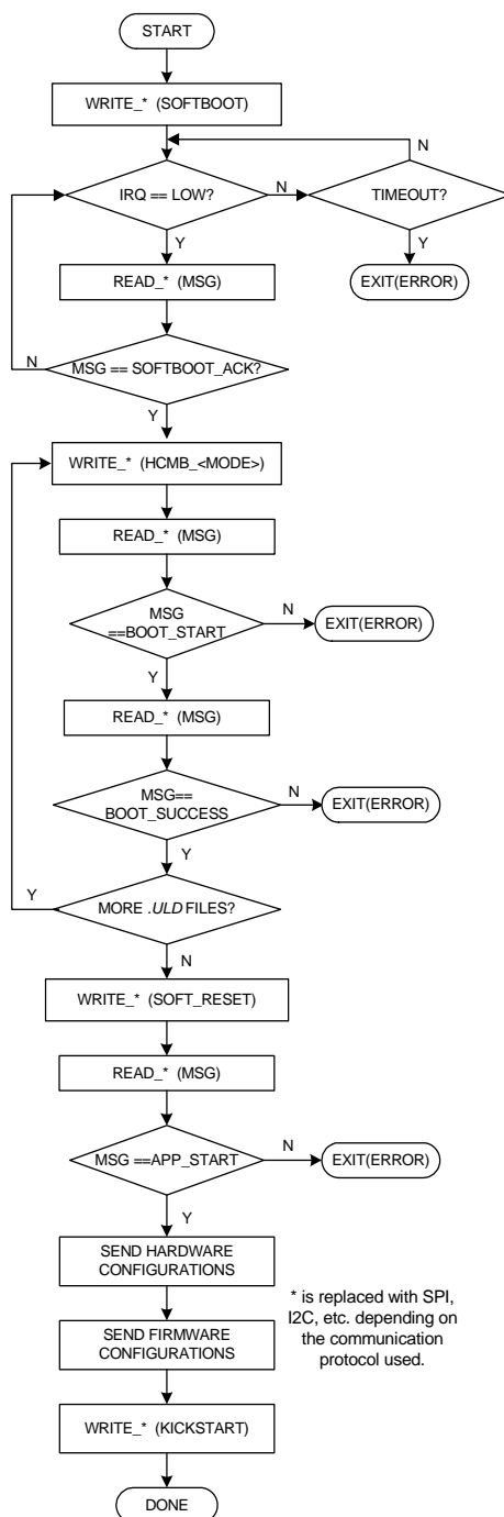
Figure 2-6. Soft Boot Example Flowchart
