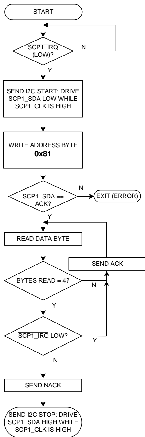
Figure 3-9. I 2 C Read Flow Diagram
