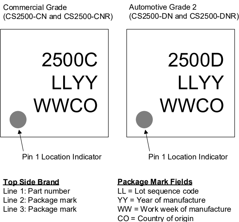
Figure 11-1. Package Marking
