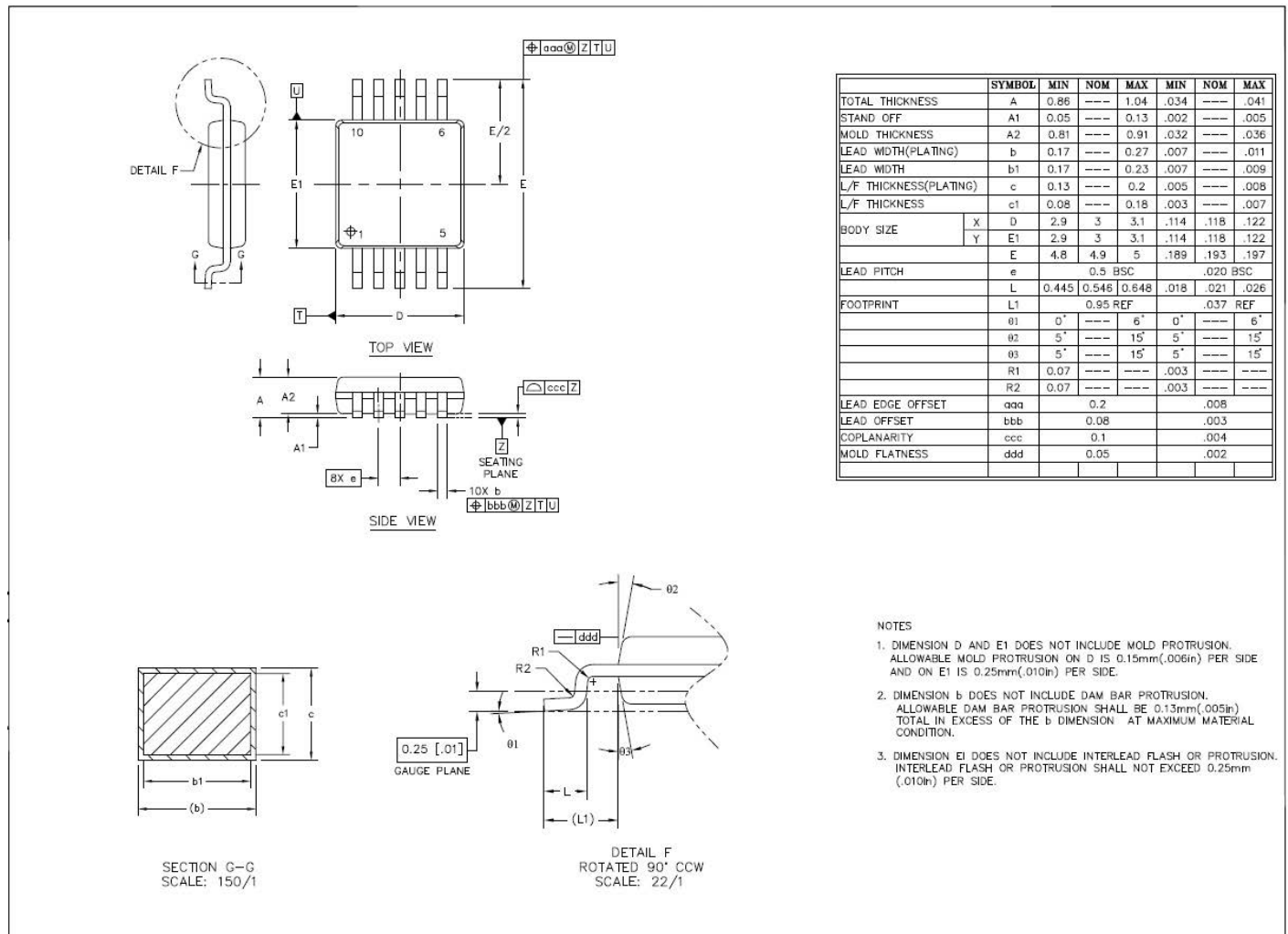
Figure 10-1. TSSOP Package Dimensions
