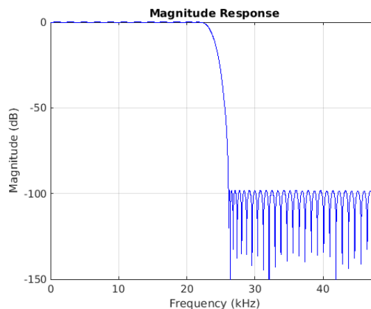
Figure 8-8. Stopband Magnitude
