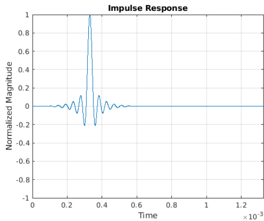
Figure 8-81. Impulse Response—Linear Phase
