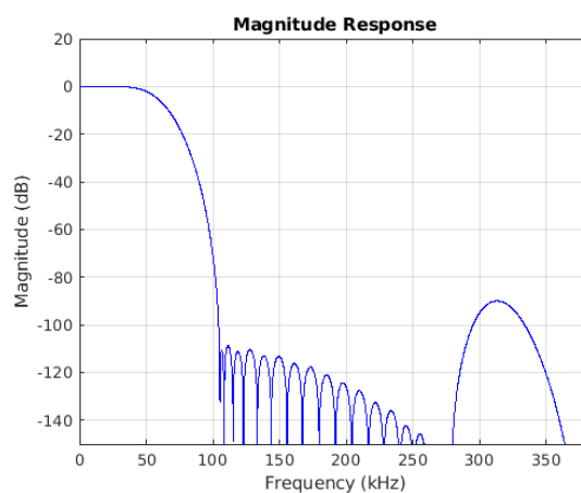
Figure 8-116. Stopband Magnitude
