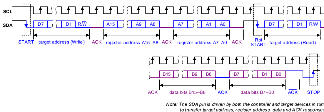
Figure 4-20. Control Interface I 2 C Register Read
