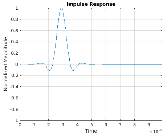
Figure 8-111. Impulse Response—Linear Phase
