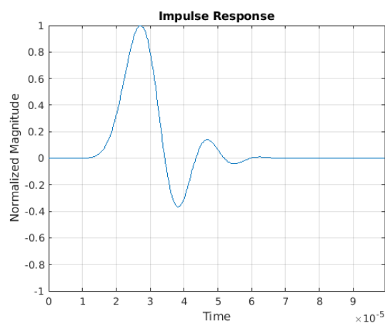
Figure 8-118. Impulse Response—Minimum Phase
