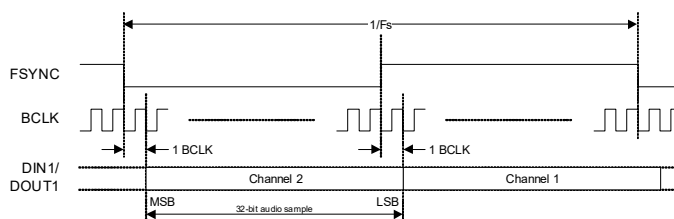
Figure 4-18. Reverse Channel Order
