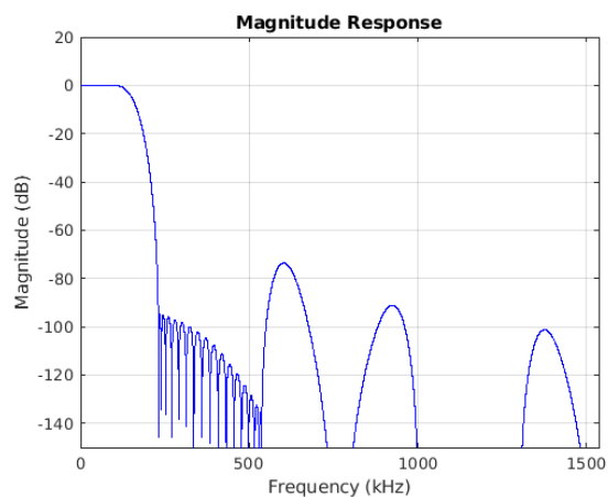
Figure 8-134. Stopband Magnitude
