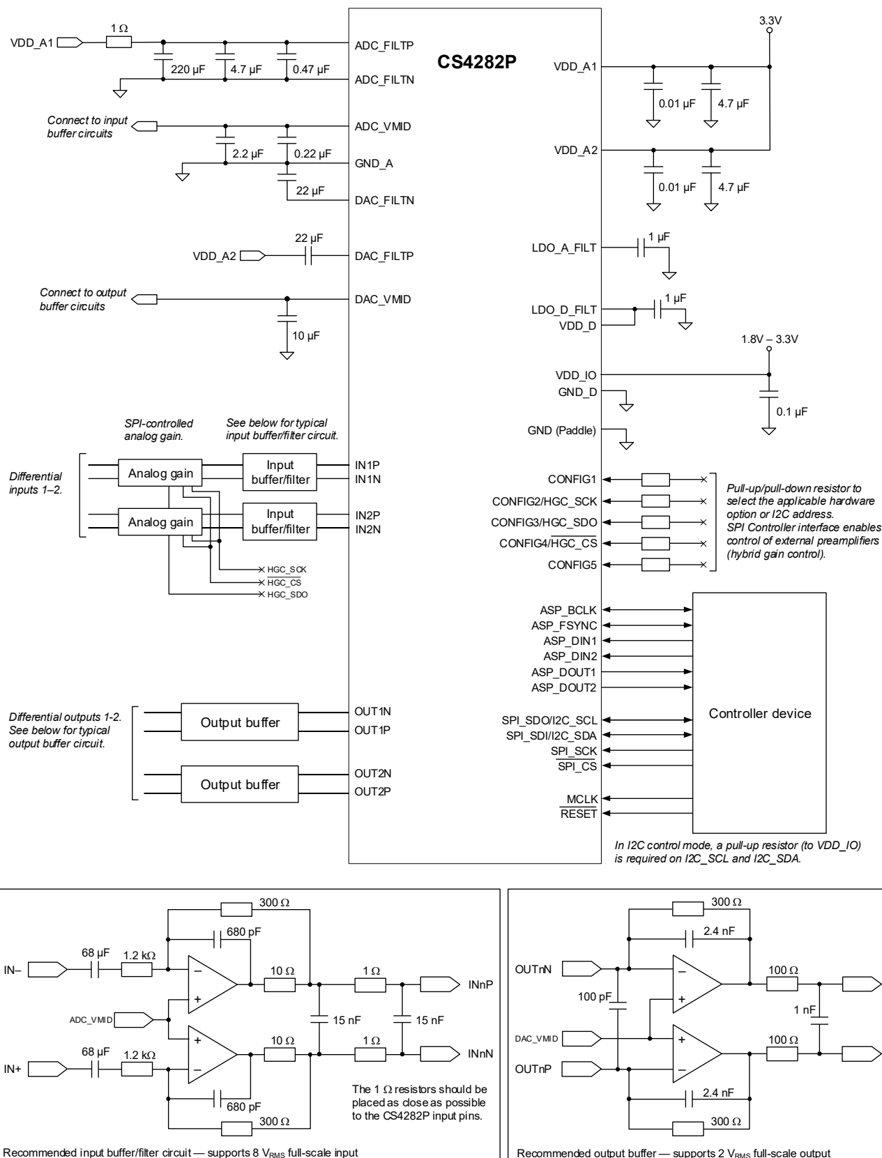
Figure 2-1. Typical Connections—Using Internal VMID Reference
