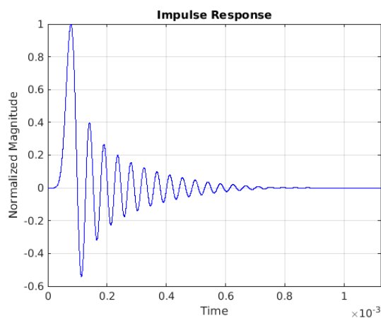
Figure 8-10. Impulse Response—Minimum Phase
