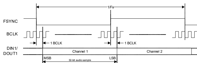
Figure 4-17. Default Channel Order
