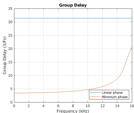
Figure 8-72. Group Delay vs. Frequency
