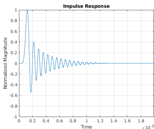
Figure 8-70. Impulse Response—Minimum Phase
