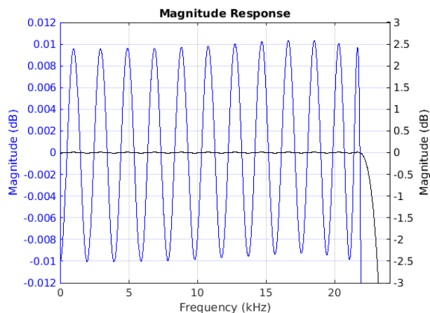
Figure 8-7. Passband Magnitude
