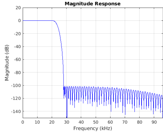
Figure 8-80. Stopband Magnitude
