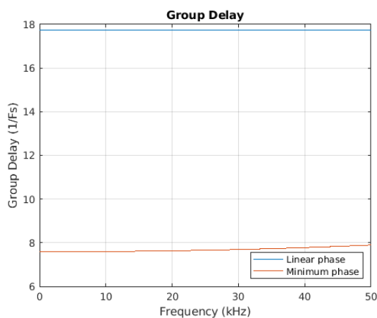
Figure 8-138. Group Delay vs. Frequency
