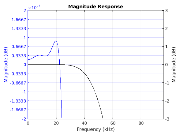
Figure 8-115. Passband Magnitude
