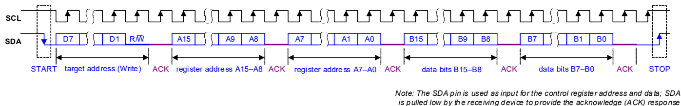
Figure 4-19. Control Interface I 2 C Register Write
