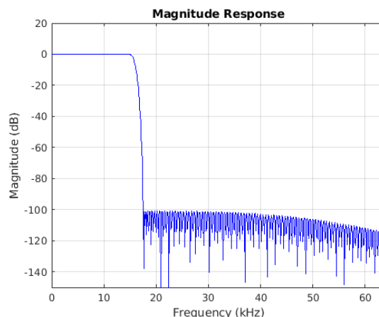
Figure 8-68. Stopband Magnitude
