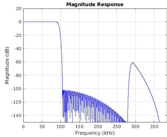
Figure 8-104. Stopband Magnitude
