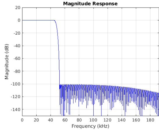
Figure 8-86. Stopband Magnitude
