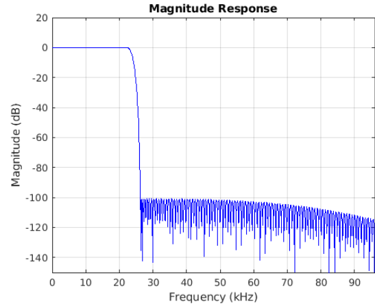
Figure 8-74. Stopband Magnitude
