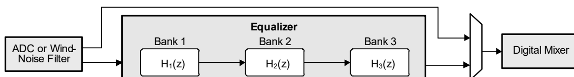
Figure 4-5. Three-Band Equalizer
