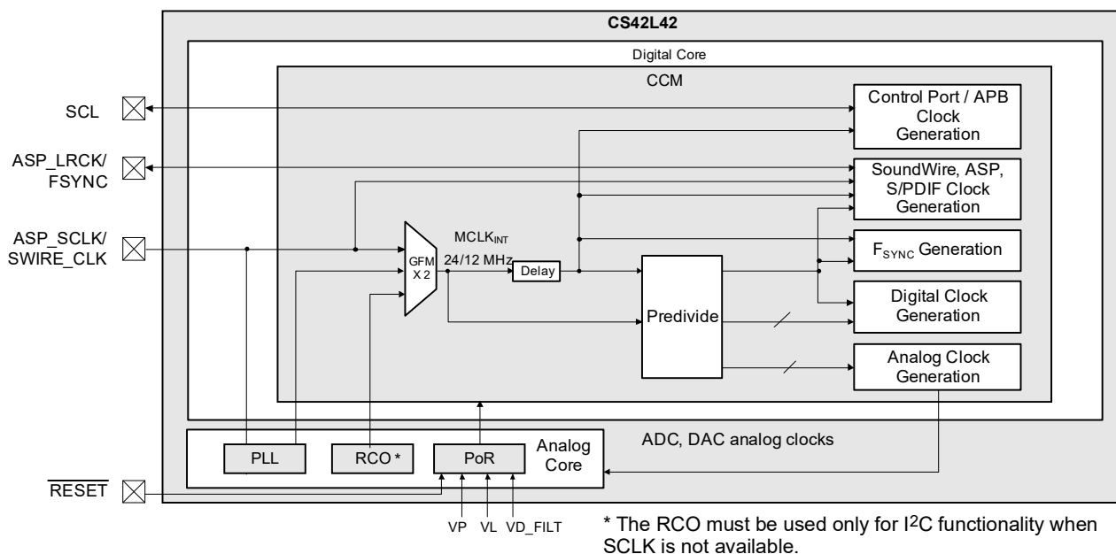
Figure 4-20. Clock Architecture Block Diagram
