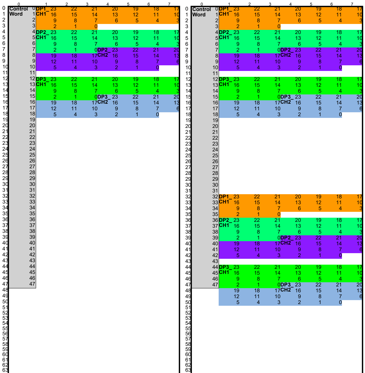
Ex. 4-3: 48-kHz Sample Interval Rate
