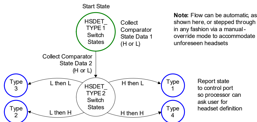
Figure 4-44. Automatic Headset Detect Flowchart
