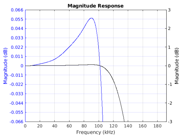
Figure 8-55. Passband Magnitude
