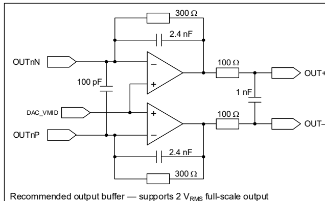
Figure 2-1. Typical Connections
