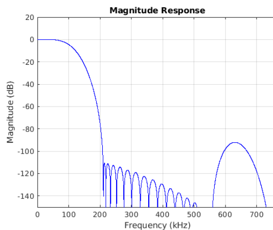
Figure 8-62. Stopband Magnitude
