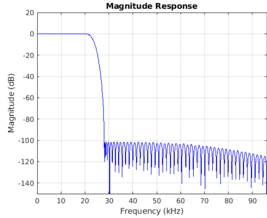
Figure 8-14. Stopband Magnitude
