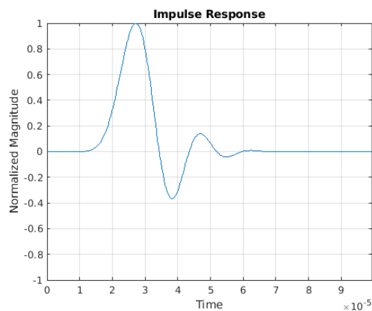
Figure 8-52. Impulse Response—Minimum Phase
