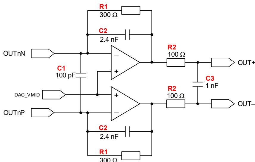
Figure 5-1. Differential Output Buffer
