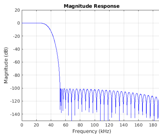
Figure 8-32. Stopband Magnitude
