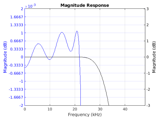
Figure 8-31. Passband Magnitude
