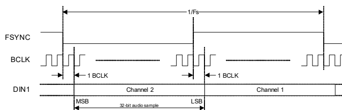
Figure 4-15. Reverse Channel Order
