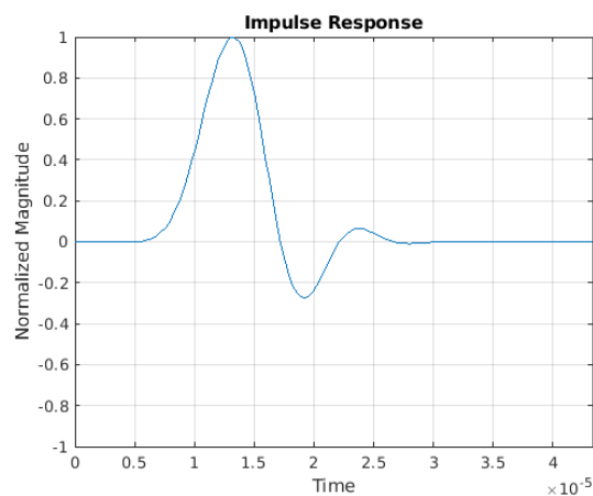
Figure 8-64. Impulse Response—Minimum Phase
