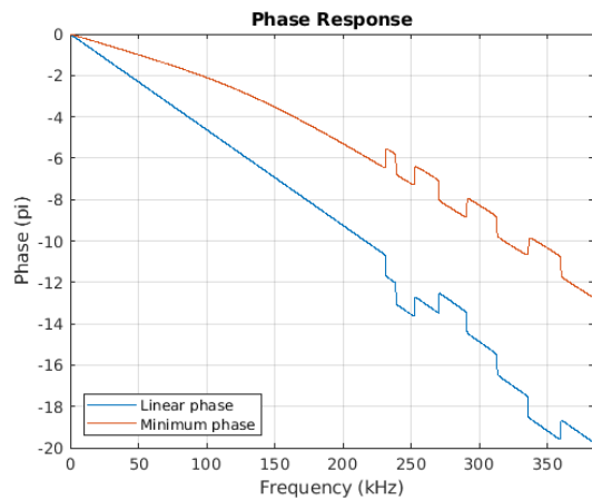
Figure 8-71. Phase vs. Frequency
