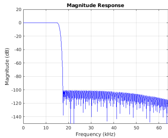
Figure 8-2. Stopband Magnitude
