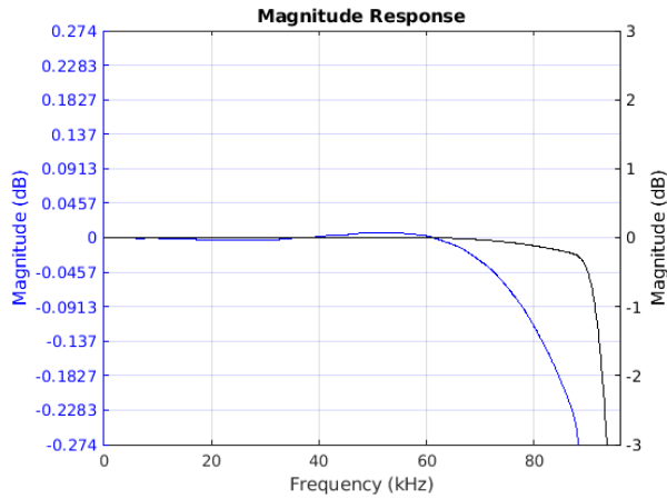
Figure 8-37. Passband Magnitude
