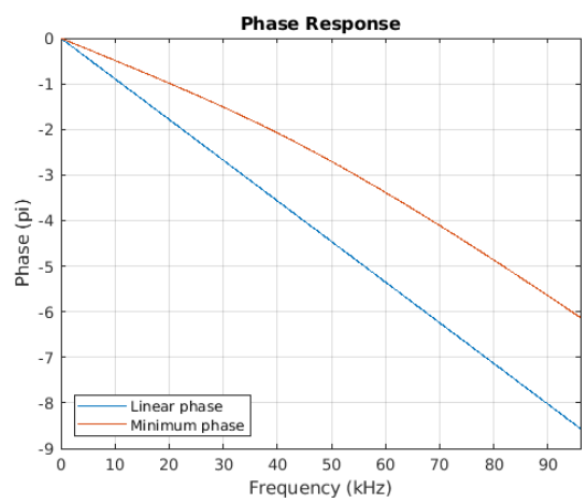
Figure 8-53. Phase vs. Frequency
