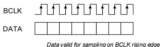
Figure 4-8. Noninverted BCLK
