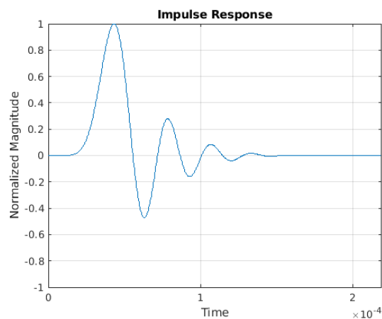
Figure 8-34. Impulse Response—Minimum Phase
