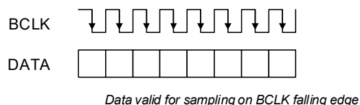
Figure 4-9. Inverted BCLK
