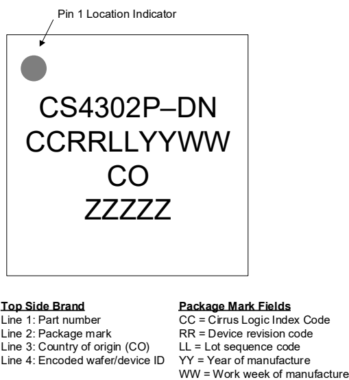
Figure 11-1. Package Marking
