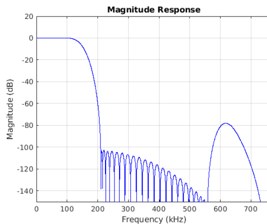
Figure 8-56. Stopband Magnitude
