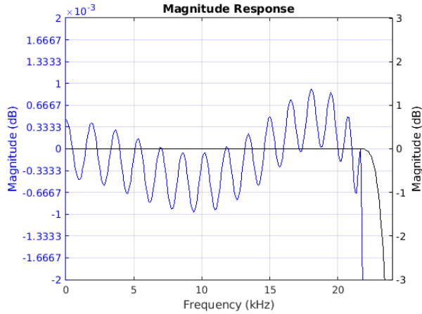
Figure 8-7. Passband Magnitude
