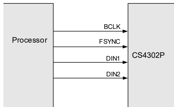
Figure 4-4. Secondary Mode
