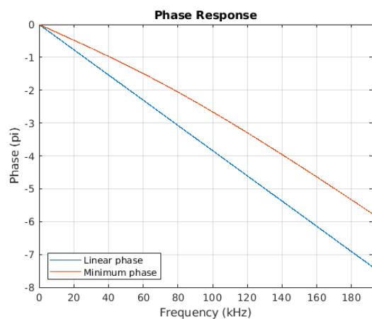
Figure 8-65. Phase vs. Frequency
