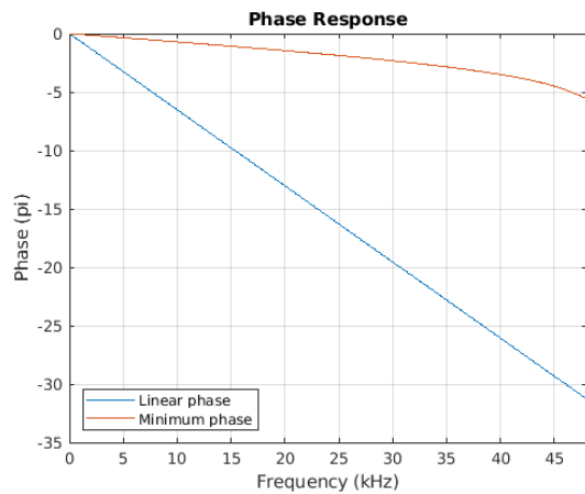
Figure 8-23. Phase vs. Frequency
