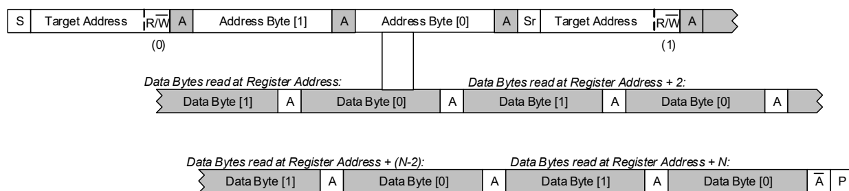
Figure 4-25. Multiple-Register Read from Specified Address
