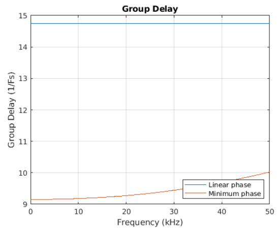
Figure 8-78. Group Delay vs. Frequency
