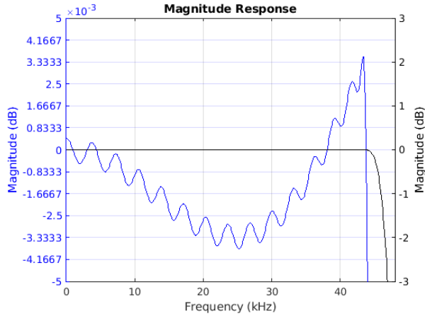
Figure 8-19. Passband Magnitude
