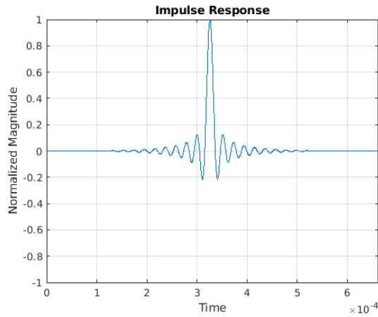
Figure 8-21. Impulse Response—Linear Phase
