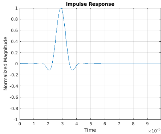
Figure 8-45. Impulse Response—Linear Phase
