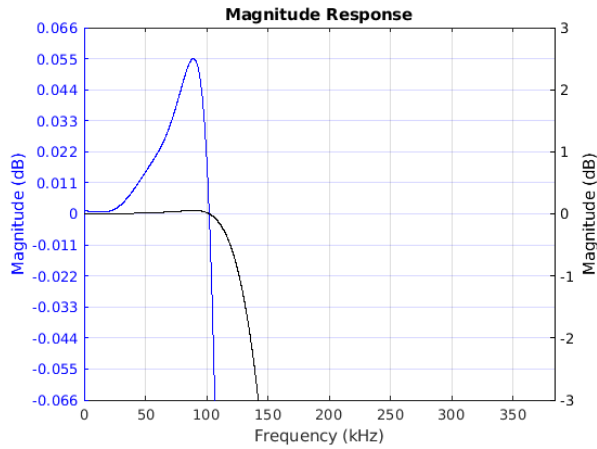
Figure 8-67. Passband Magnitude
