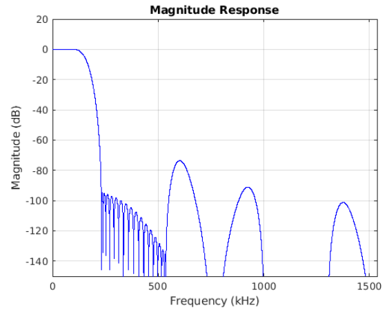
Figure 8-68. Stopband Magnitude
