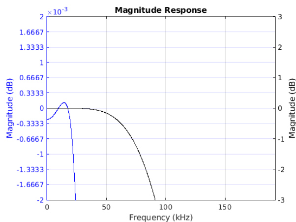
Figure 8-61. Passband Magnitude
