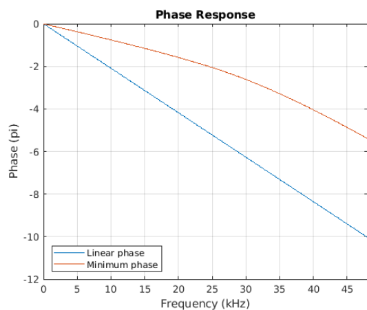
Figure 8-35. Phase vs. Frequency
