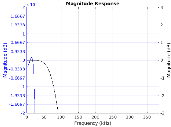
Figure 8-73. Passband Magnitude
