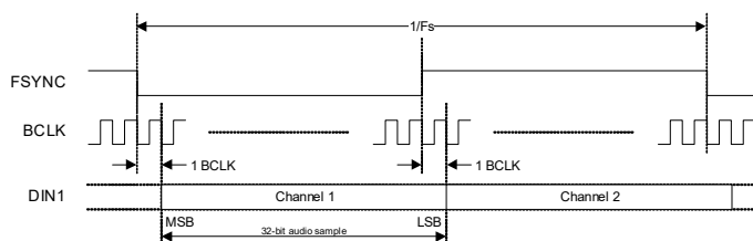
Figure 4-14. Default Channel Order
