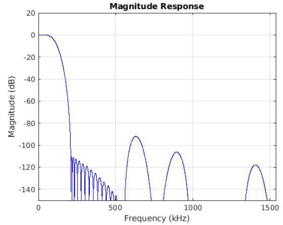
Figure 8-74. Stopband Magnitude
