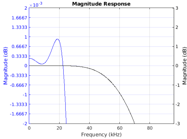
Figure 8-43. Passband Magnitude
