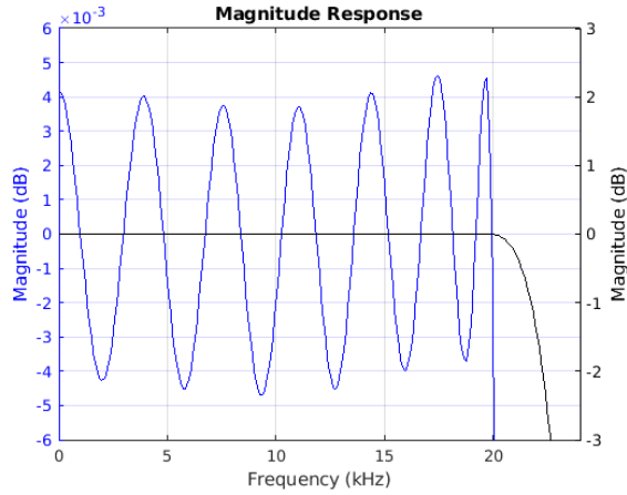
Figure 8-13. Passband Magnitude
