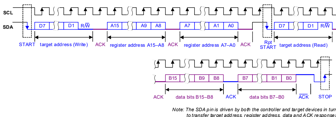
Figure 4-21. Control Interface I 2 C Register Read
