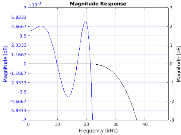
Figure 8-25. Passband Magnitude
