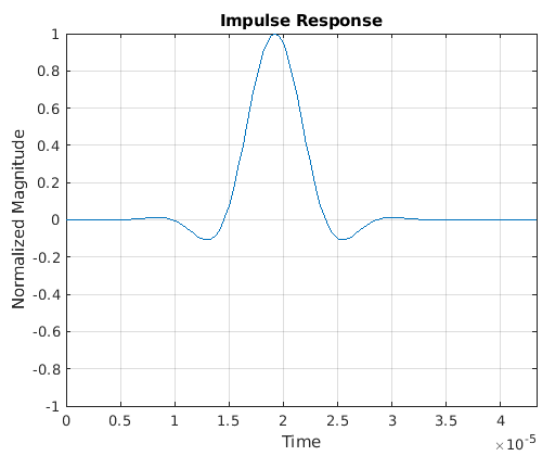
Figure 8-63. Impulse Response—Linear Phase
