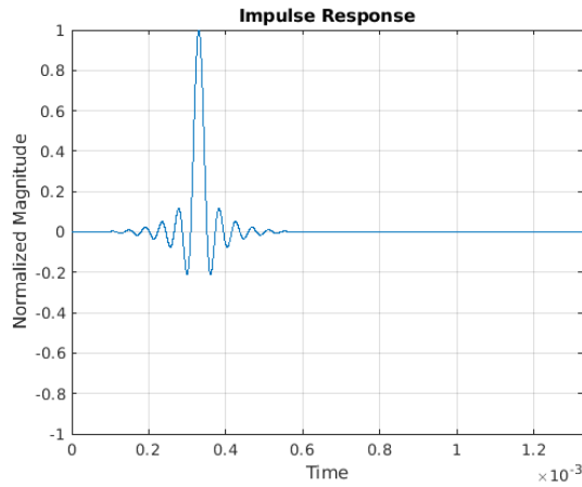
Figure 8-15. Impulse Response—Linear Phase
