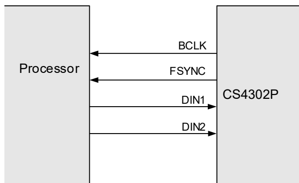
Figure 4-3. Primary Mode
