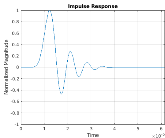
Figure 8-58. Impulse Response—Minimum Phase
