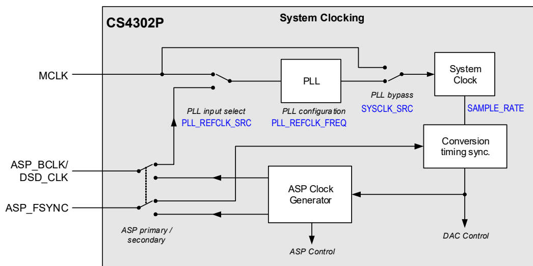
Figure 4-1. System Clocking
