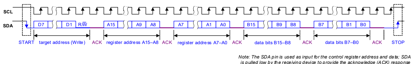
Figure 4-20. Control Interface I 2 C Register Write
