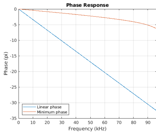
Figure 8-41. Phase vs. Frequency
