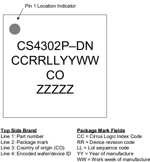
Figure 11-1. Package Marking
