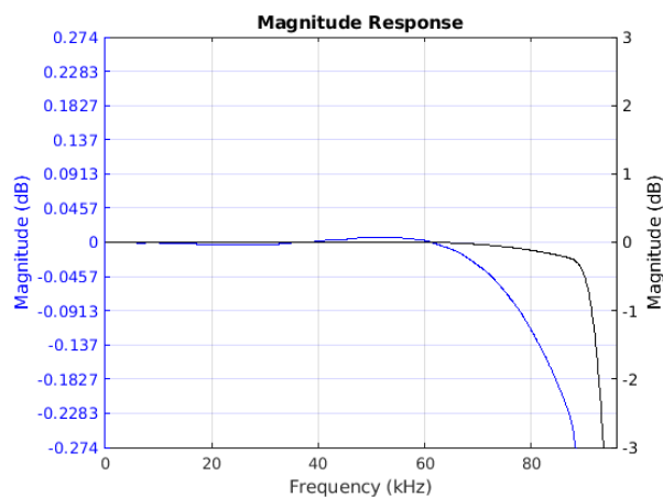
Figure 8-37. Passband Magnitude
