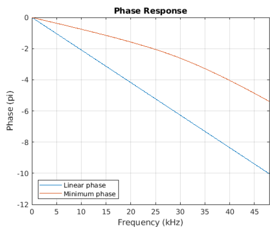
Figure 8-35. Phase vs. Frequency
