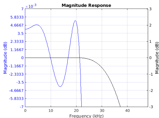
Figure 8-25. Passband Magnitude
