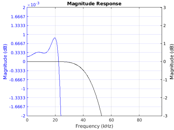
Figure 8-49. Passband Magnitude
