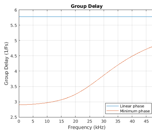
Figure 8-30. Group Delay vs. Frequency
