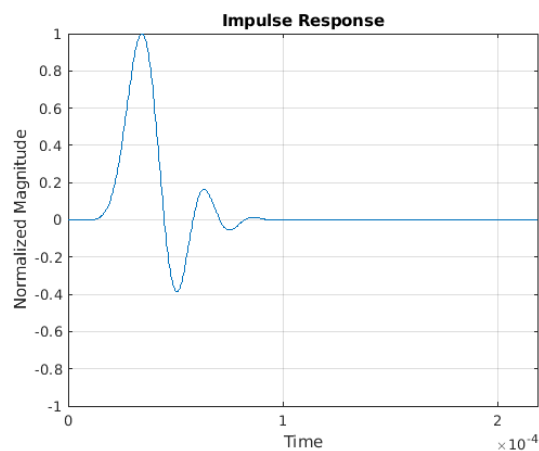
Figure 8-28. Impulse Response—Minimum Phase
