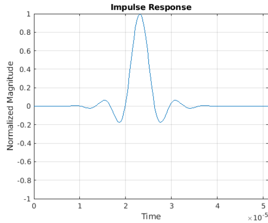
Figure 8-69. Impulse Response—Linear Phase
