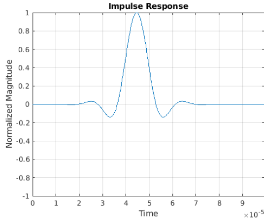
Figure 8-51. Impulse Response—Linear Phase
