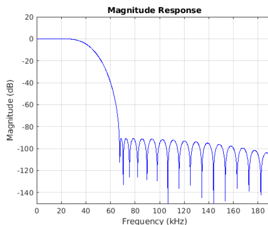
Figure 8-26. Stopband Magnitude
