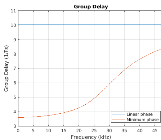
Figure 8-36. Group Delay vs. Frequency
