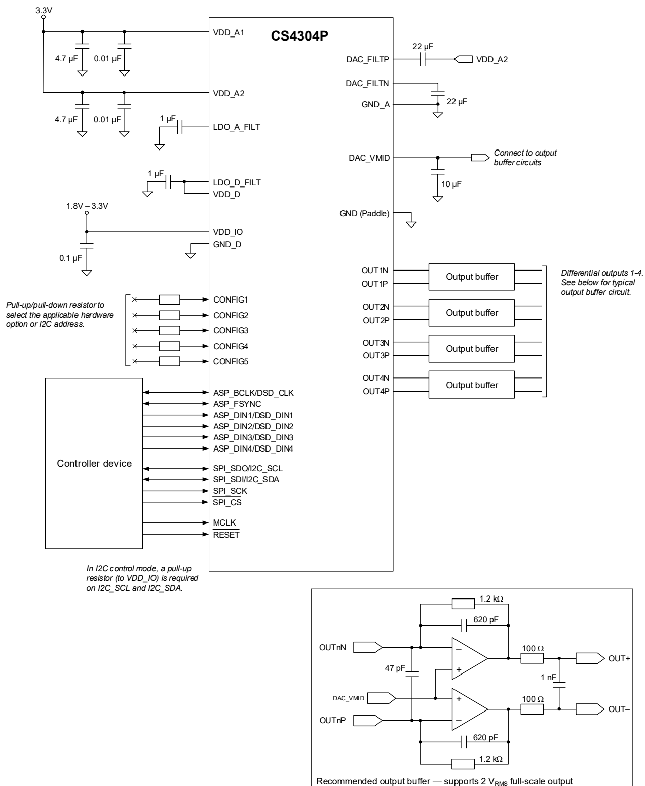
Figure 2-1. Typical Connections
