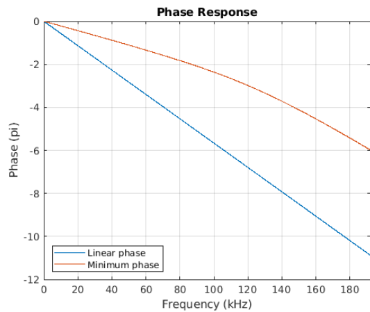
Figure 8-59. Phase vs. Frequency
