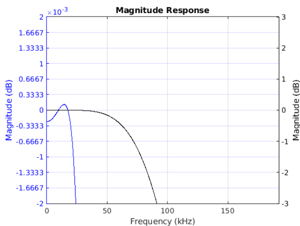
Figure 8-61. Passband Magnitude
