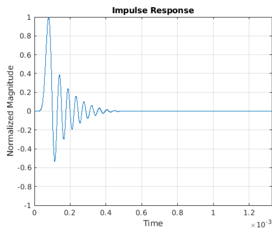
Figure 8-16. Impulse Response—Minimum Phase
