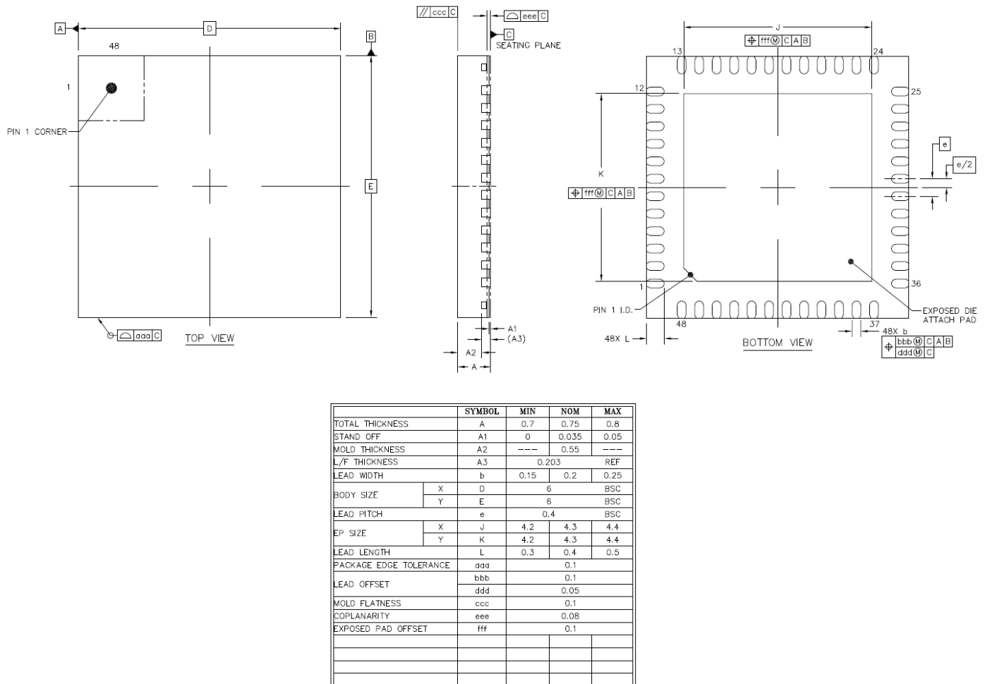
Figure 10-1. QFN Package Drawing
