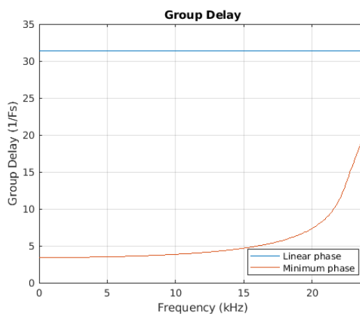
Figure 8-12. Group Delay vs. Frequency
