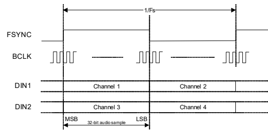
Figure 4-23. Left-Justified Data Format
