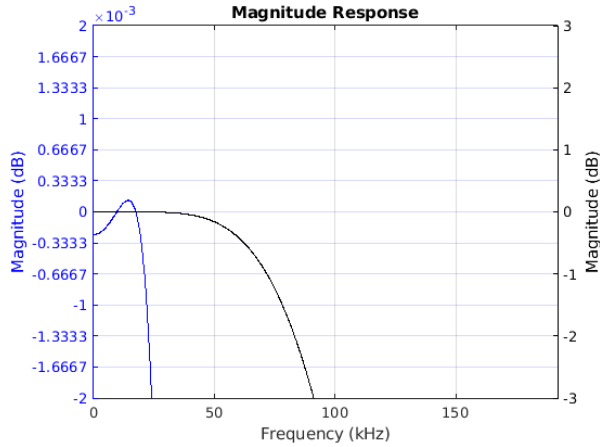
Figure 8-61. Passband Magnitude
