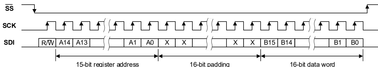
Figure 4-46. Control Interface SPI Register Write
