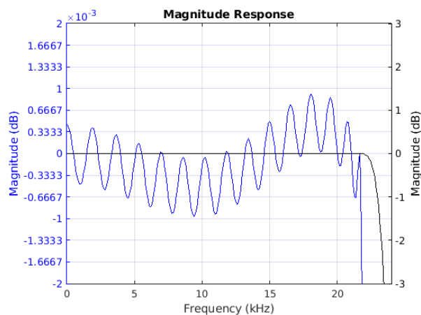
Figure 8-7. Passband Magnitude
