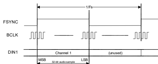
Figure 4-32. Left-Justified Data Format
