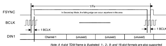
Figure 4-33. TDM Data Format
