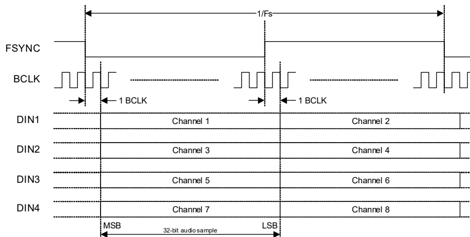
Figure 4-12. I 2 S Data Format
