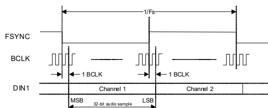
Figure 4-27. I 2 S Data Format
