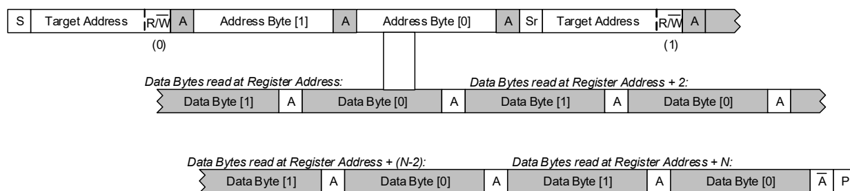
Figure 4-45. Multiple-Register Read from Specified Address
