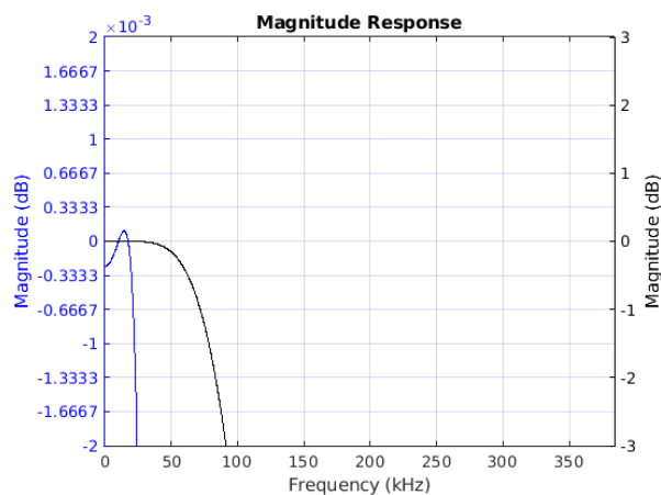
Figure 8-73. Passband Magnitude
