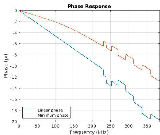
Figure 8-71. Phase vs. Frequency
