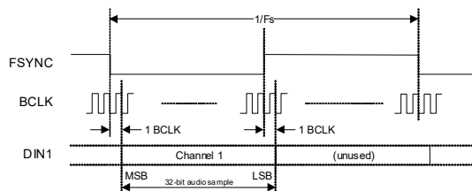
Figure 4-31. I 2 S Data Format
