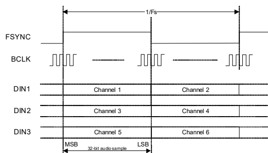
Figure 4-18. Left-Justified Data Format
