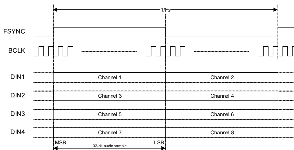
Figure 4-13. Left-Justified Data Format
