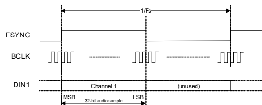
Figure 4-32. Left-Justified Data Format
