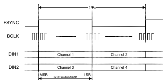
Figure 4-23. Left-Justified Data Format
