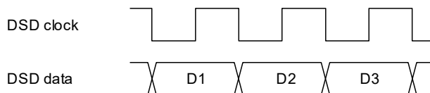
Figure 4-37. DSD Interface Timing
