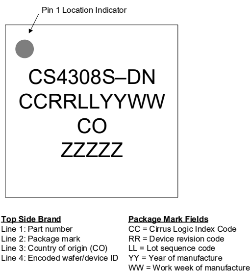
Figure 11-1. Package Marking
