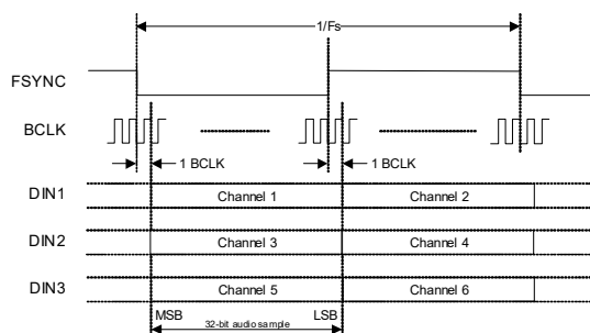
Figure 4-17. I2S Data Format
