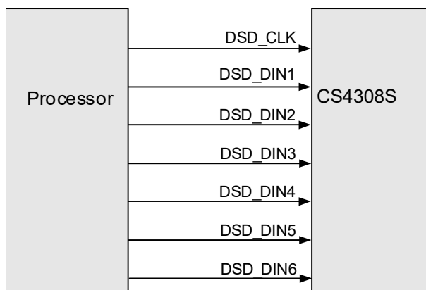
Figure 4-36. DSD Interface Connection
