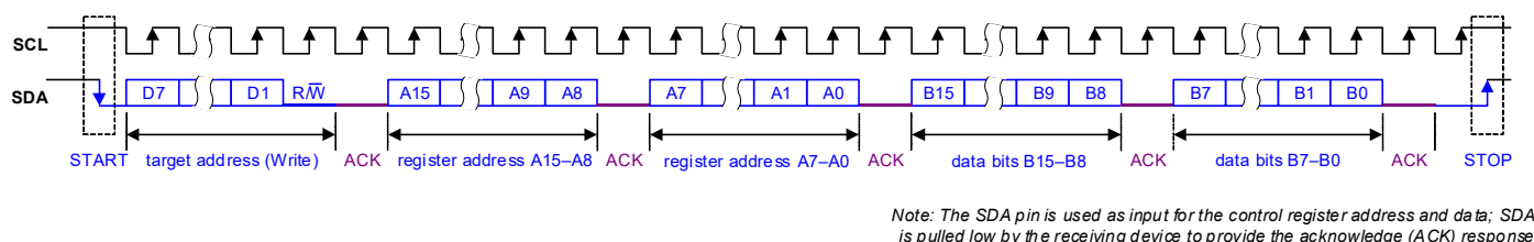
Figure 4-40. Control Interface I 2 C Register Write
