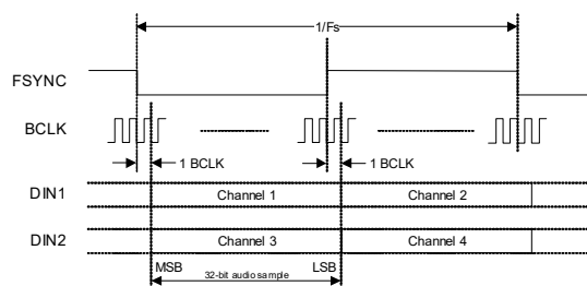
Figure 4-22. I2S Data Format
