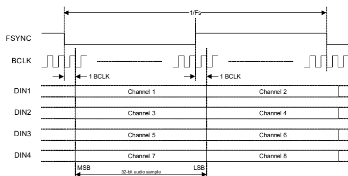
Figure 4-34. Default Channel Order
