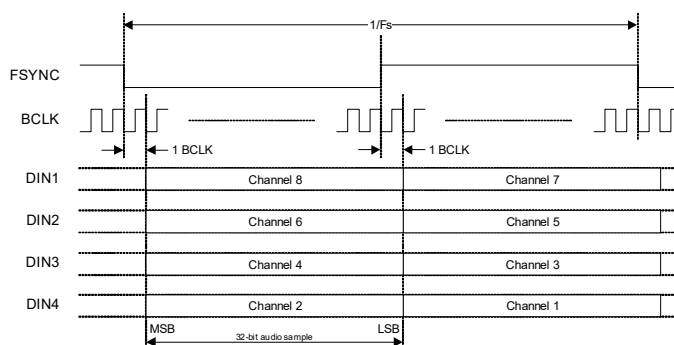
Figure 4-35. Reverse Channel Order
