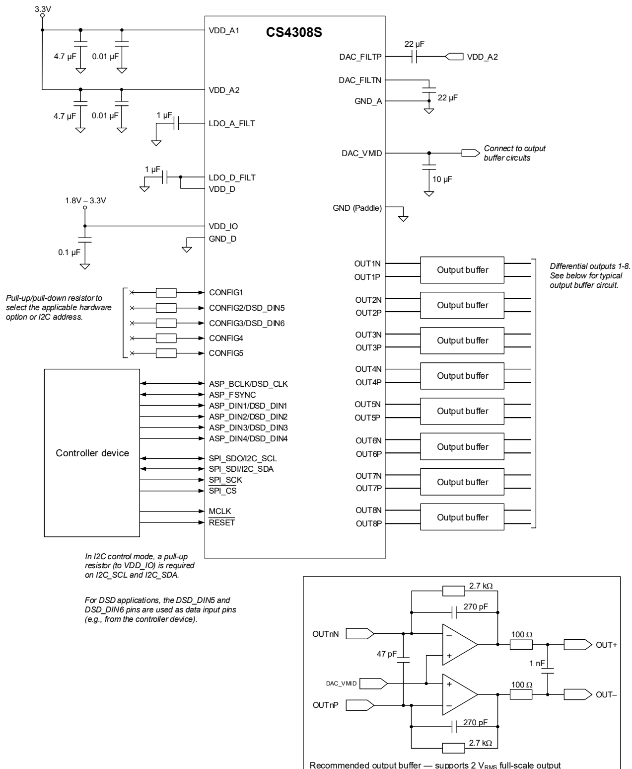
Figure 2-1. Typical Connections
