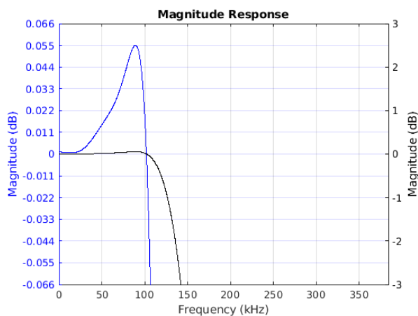
Figure 8-67. Passband Magnitude
