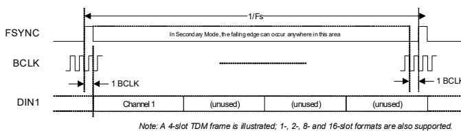
Figure 4-33. TDM Data Format
