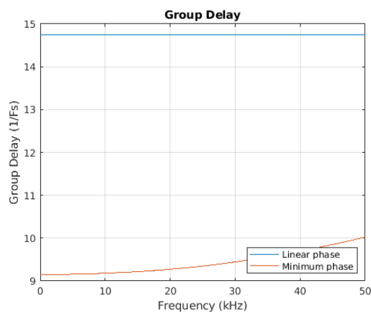
Figure 8-78. Group Delay vs. Frequency
