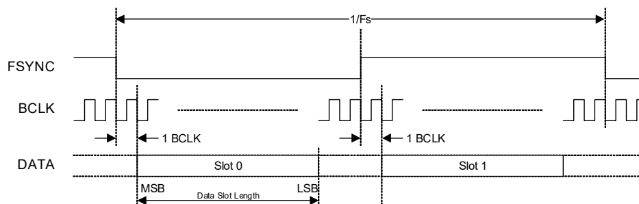
Figure 4-7. I 2 S Data Format
