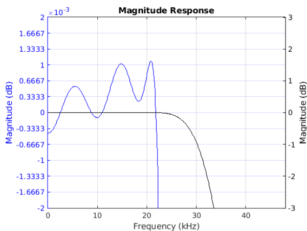
Figure 8-31. Passband Magnitude
