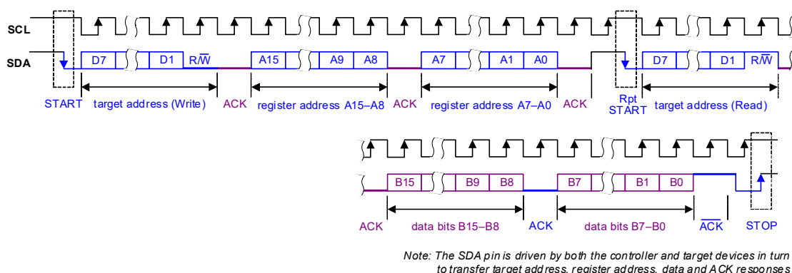
Figure 4-41. Control Interface I 2 C Register Read
