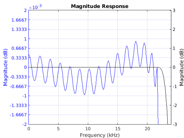
Figure 8-7. Passband Magnitude
