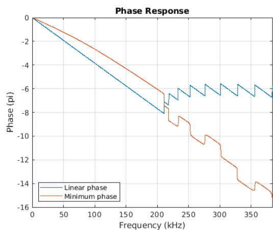
Figure 8-77. Phase vs. Frequency
