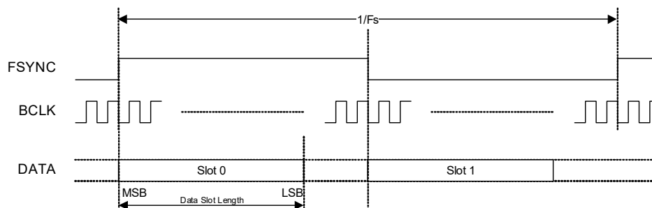
Figure 4-8. Left-Justified Data Format
