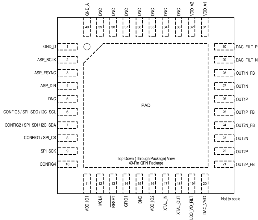
Figure 1-1. QFN 40-Pin Diagram (Top View, Through Package)
