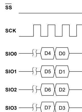
Figure 4-35. Dummy Data—4-bit Mode
