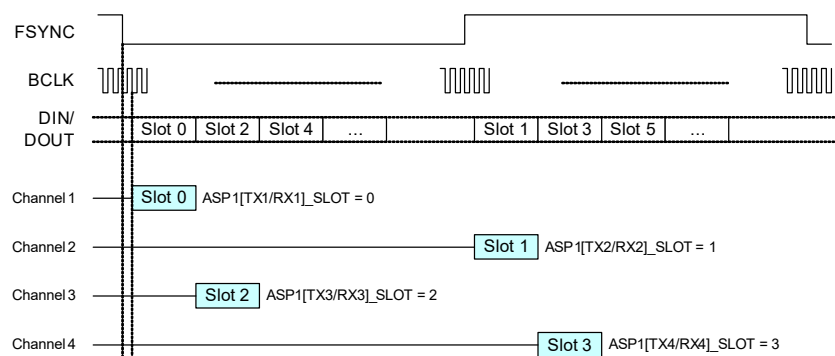
Figure 4-47. I 2 S Example
