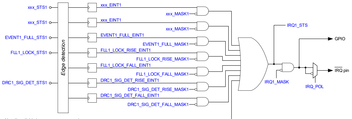
Figure 4-54. Interrupt Controller
