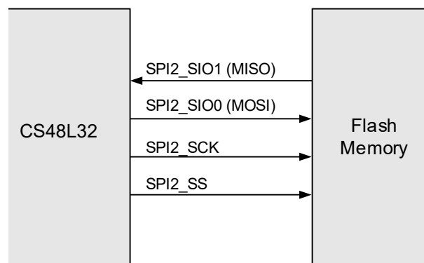
Figure 4-31. 4-Wire Mode
