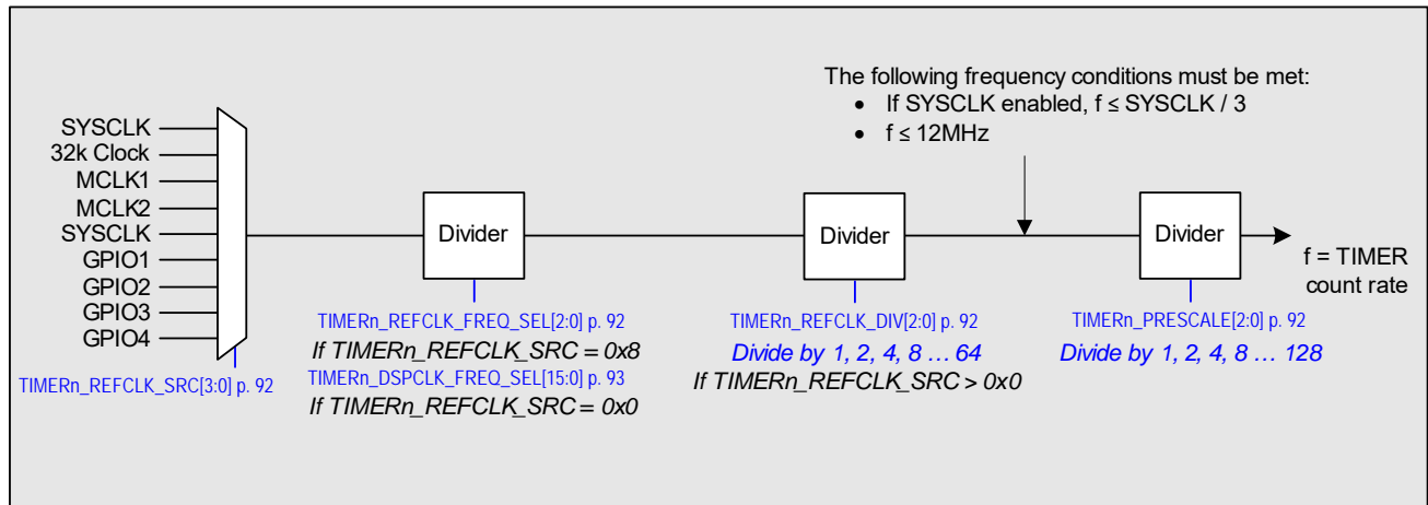
Figure 4-28. General-Purpose Timer
