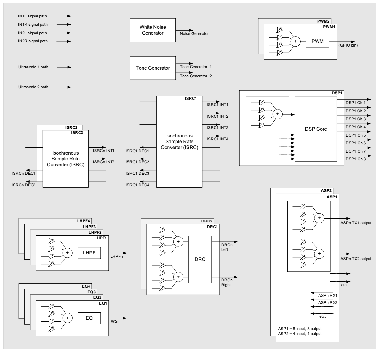
Figure 4-15. Digital Core
