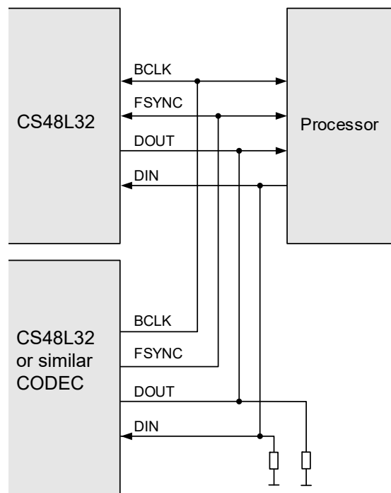
Figure 4-50. ASP Operation with Other Codec as Master
