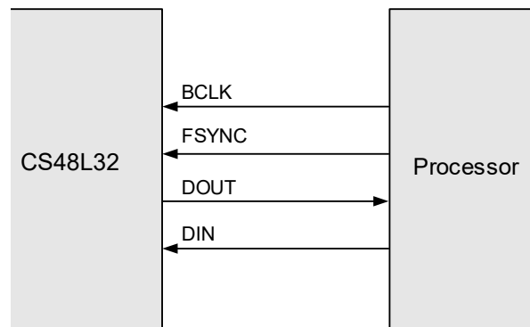
Figure 4-40. Slave Mode
