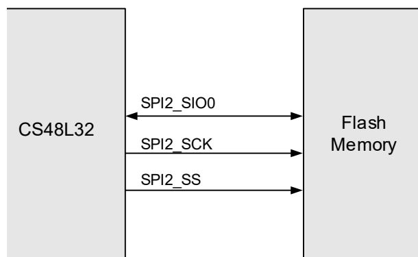
Figure 4-30. 3-Wire Mode
