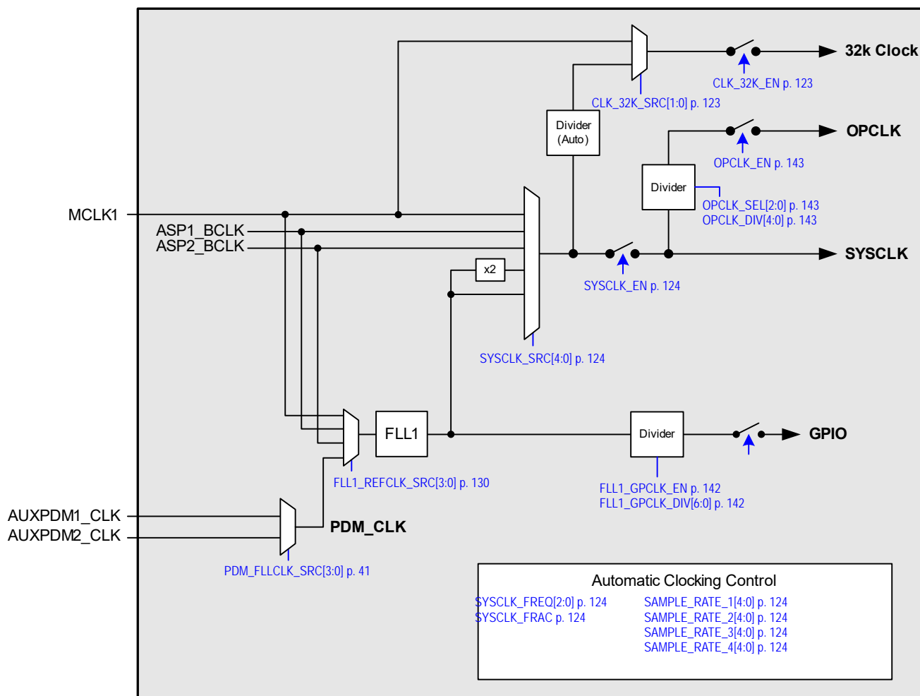
Figure 4-52. System Clocking
