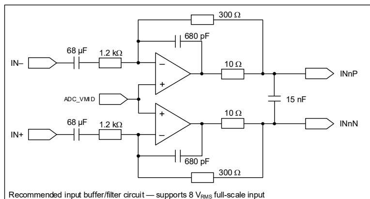
Figure 2-1. Typical Connections—Using Internal VMID Reference
