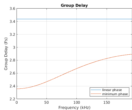
Figure 8-54. Group Delay vs. Frequency
