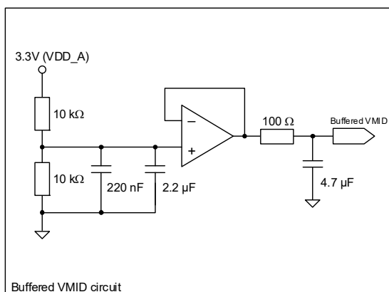
Figure 2-2. Typical Connections—Using External VMD Reference
