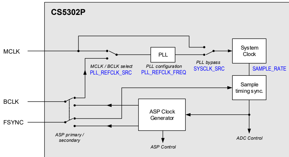
Figure 4-1. System Clocking
