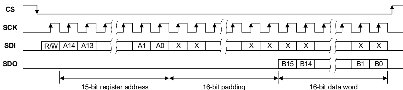
Figure 4-25. Control Interface SPI Register Read
