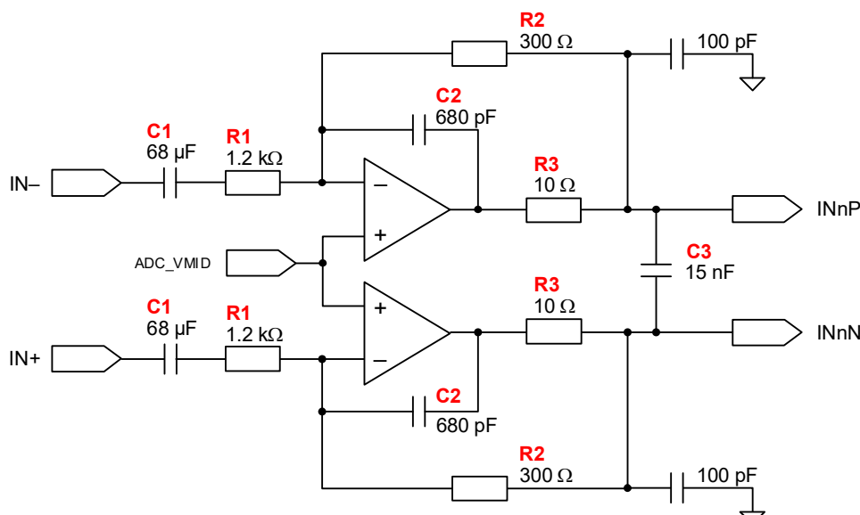
Figure 5-1. Differential Input Buffer
