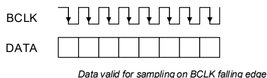
Figure 4-11. Inverted BCLK
