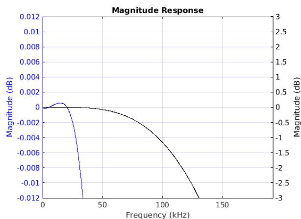
Figure 8-49. Passband Magnitude
