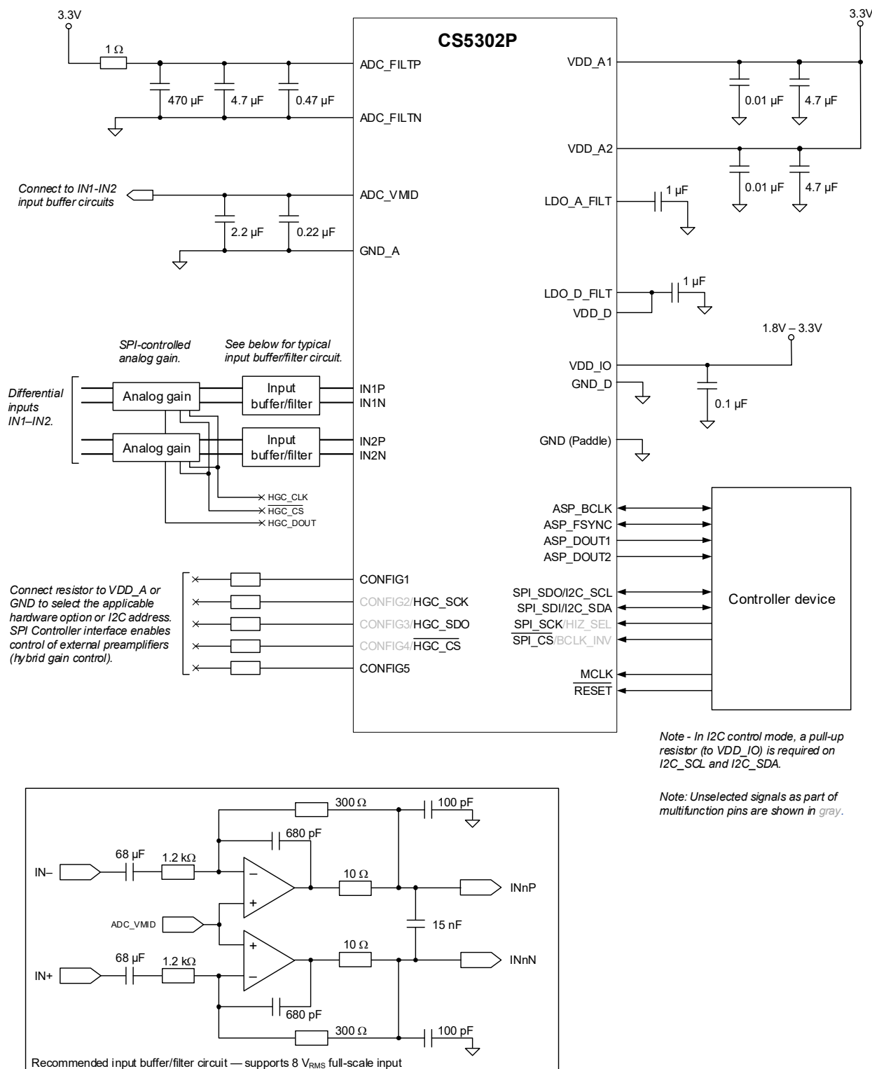
Figure 2-1. Typical Connections
