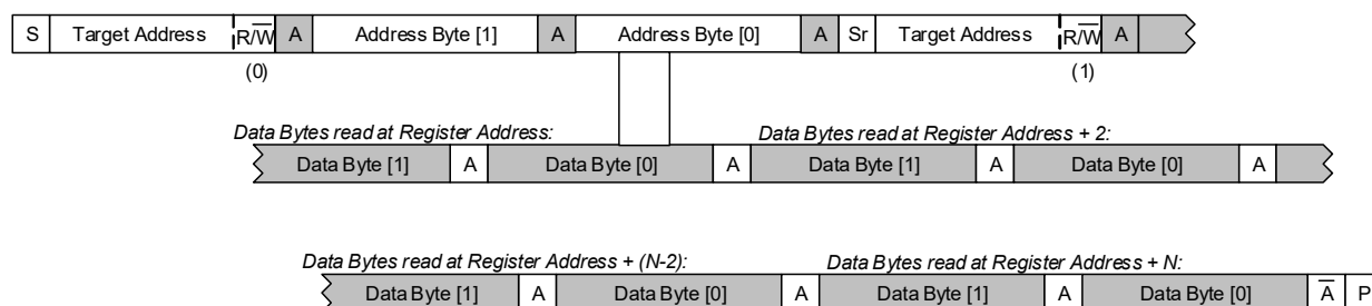
Figure 4-32. Multiple-Register Read from Specified Address
