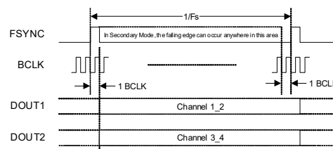
Figure 4-21. TDM Data Format—2 x DOUT
