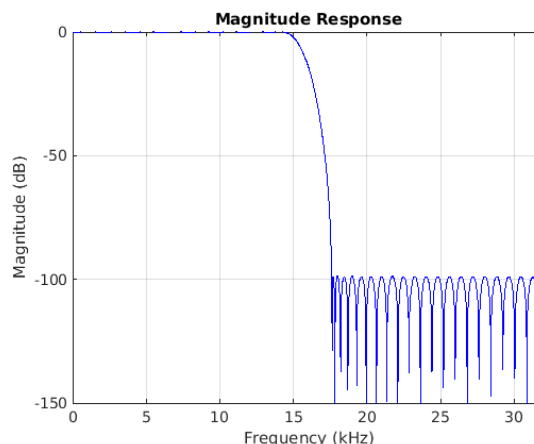
Figure 8-2. Stopband Magnitude
