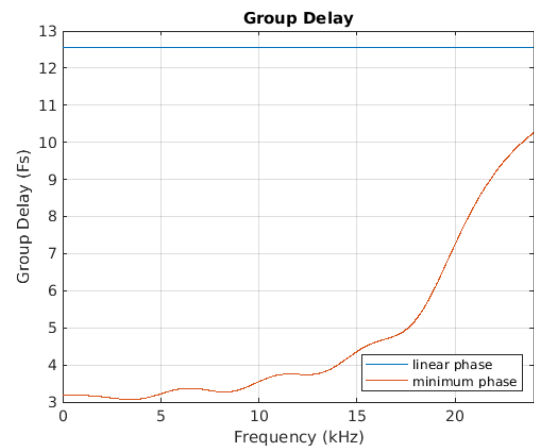
Figure 8-18. Group Delay vs. Frequency
