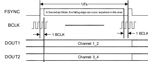
Figure 4-21. TDM Data Format—2 x DOUT
