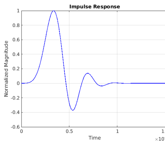
Figure 8-58. Impulse Response—Minimum Phase
