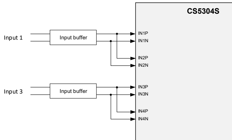
Figure 4-5. Input Summing
