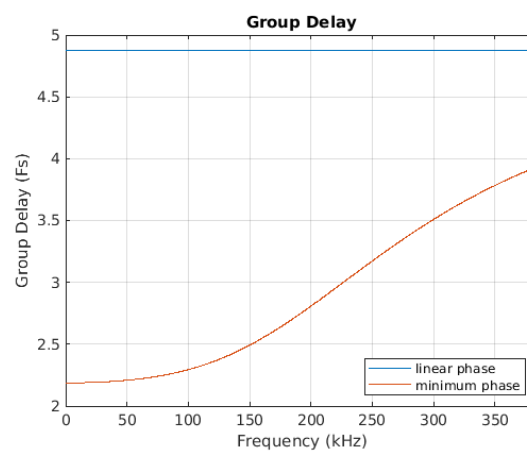
Figure 8-60. Group Delay vs. Frequency
