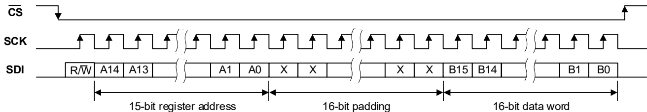
Figure 4-33. Control Interface SPI Register Write
