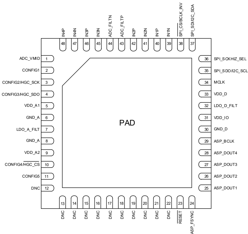
Figure 1-1. QFN 48-pin diagram (Top View, Through Package)
