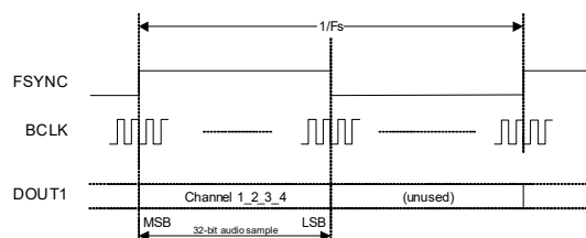
Figure 4-23. Left-Justified Data Format
