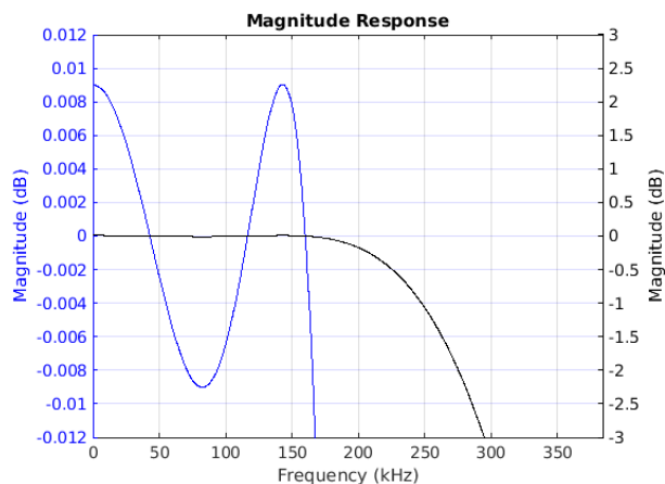
Figure 8-55. Passband Magnitude
