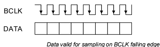
Figure 4-12. Inverted BCLK
