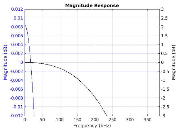
Figure 8-61. Passband Magnitude
