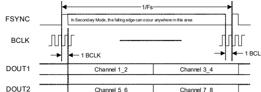
Figure 4-21. TDM Data Format—2 x DOUT
