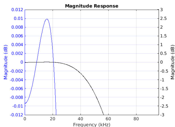
Figure 8-37. Passband Magnitude
