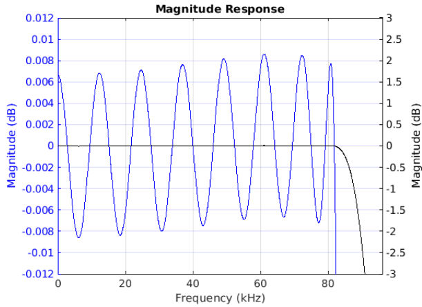
Figure 8-31. Passband Magnitude
