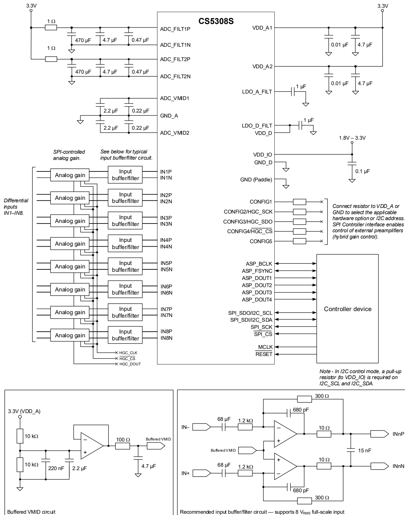
Figure 2-2. Typical Connections—Using External VMID Reference
