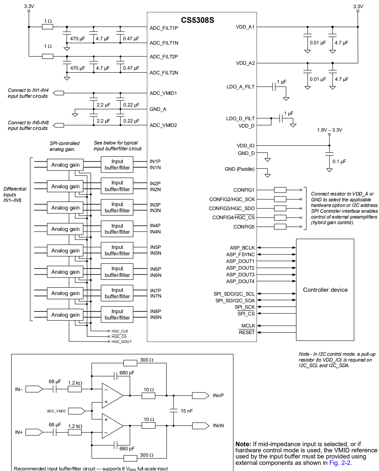
Figure 2-1. Typical Connections—Using Internal VMID Reference
