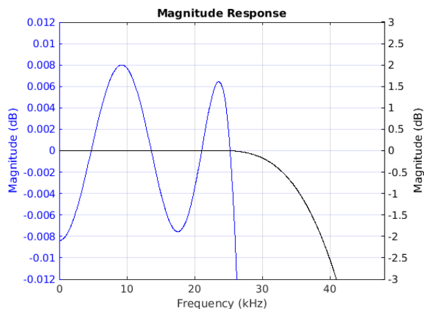
Figure 8-25. Passband Magnitude
