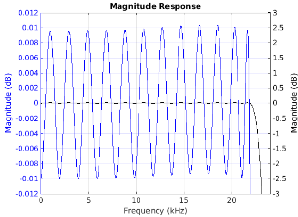
Figure 8-7. Passband Magnitude
