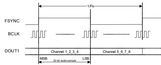
Figure 4-24. Left-Justified Data Format
