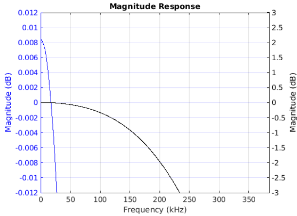
Figure 8-61. Passband Magnitude
