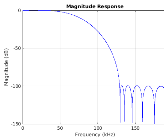
Figure 8-38. Stopband Magnitude
