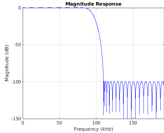
Figure 8-32. Stopband Magnitude
