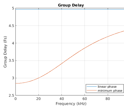
Figure 8-42. Group Delay vs. Frequency
