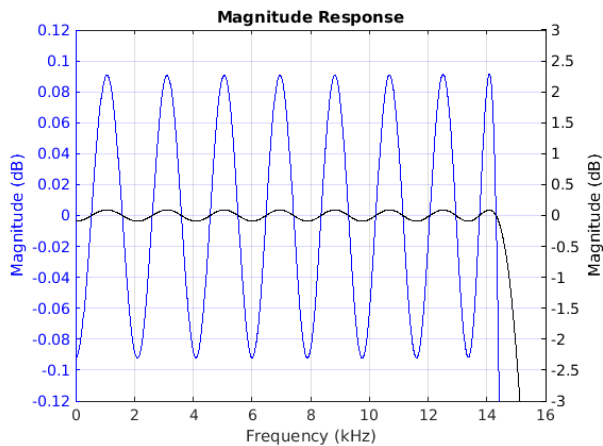
Figure 8-1. Passband Magnitude
