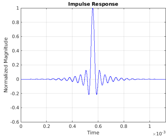
Figure 8-9. Impulse Response—Linear Phase
