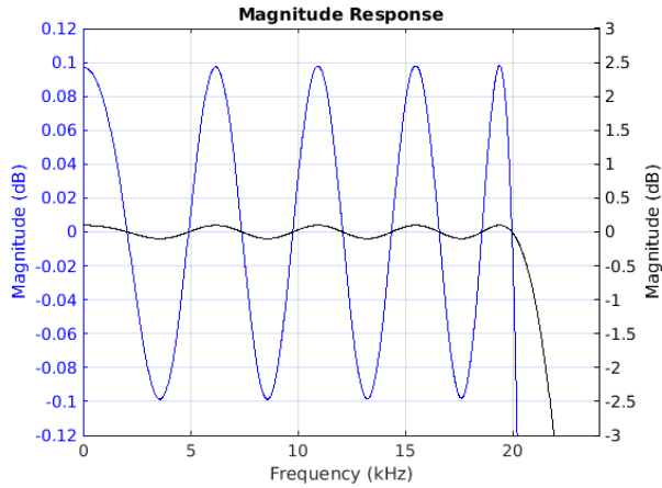
Figure 8-13. Passband Magnitude
