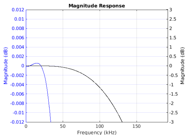
Figure 8-49. Passband Magnitude
