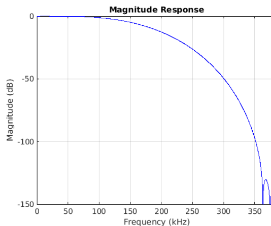
Figure 8-50. Stopband Magnitude
