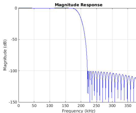
Figure 8-44. Stopband Magnitude
