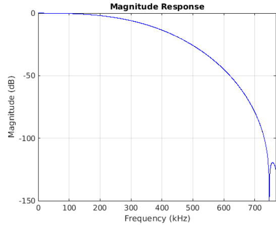
Figure 8-62. Stopband Magnitude
