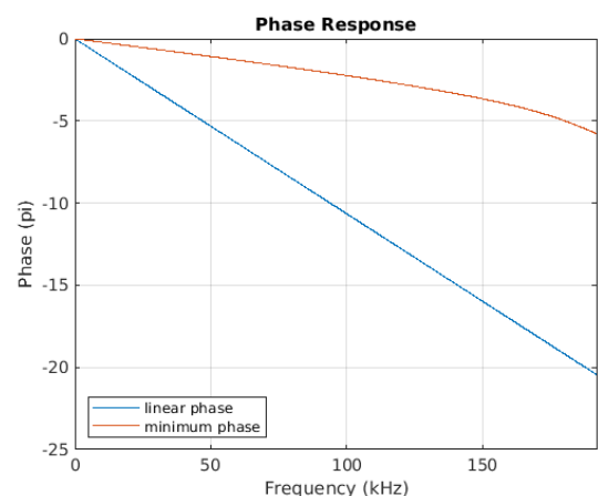
Figure 8-47. Phase vs. Frequency
