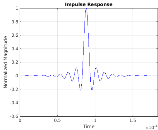
Figure 8-33. Impulse Response—Linear Phase
