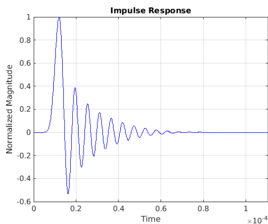
Figure 8-46. Impulse Response—Minimum Phase
