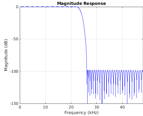
Figure 8-8. Stopband Magnitude
