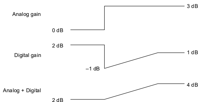
Figure 4-4. Gain Ramping
