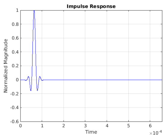
Figure 8-27. Impulse Response—Linear Phase
