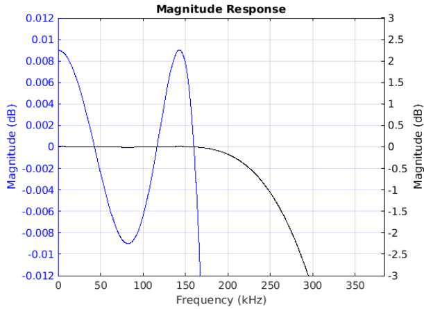
Figure 8-55. Passband Magnitude
