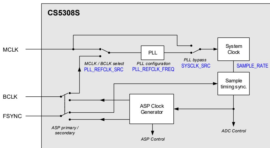
Figure 4-1. System Clocking
