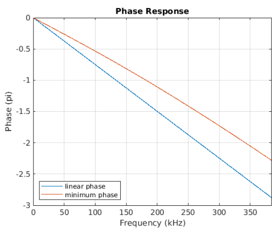
Figure 8-65. Phase vs. Frequency
