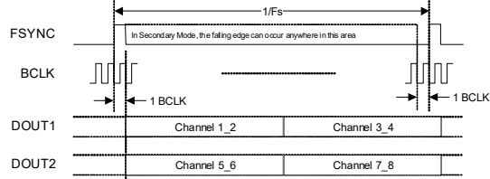
Figure 4-21. TDM Data Format—2 x DOUT
