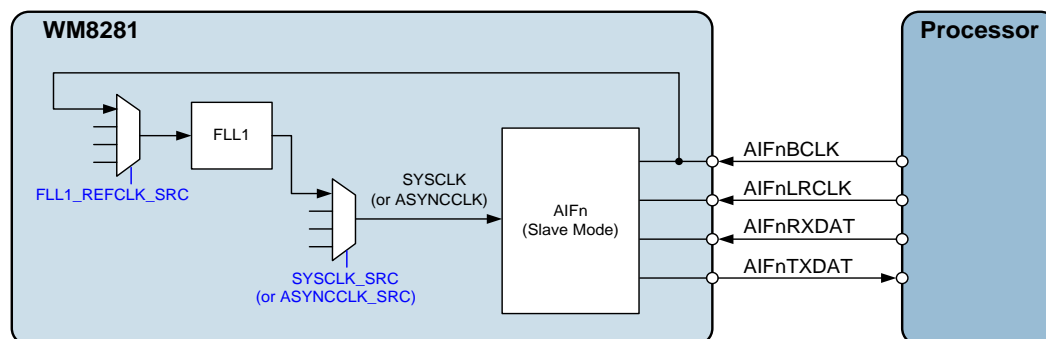
Figure 98 AIF Slave Mode, using BCLK and FLL as Reference
