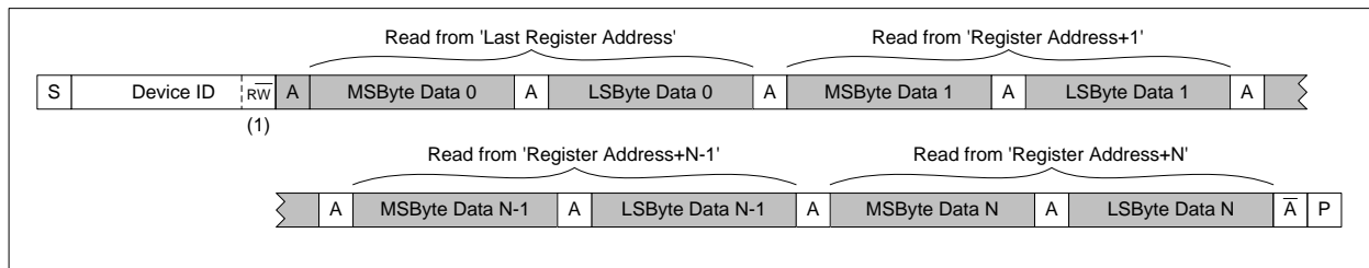
Figure 78 Multiple Register Read from Last Address using Auto-increment
