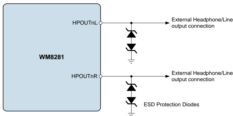
Figure 88 ESD Diode Configuration for External Output Connections
