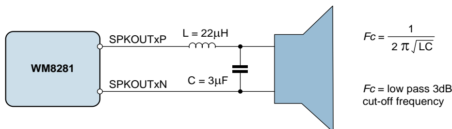
Figure 90 Class D Output Filter Components
