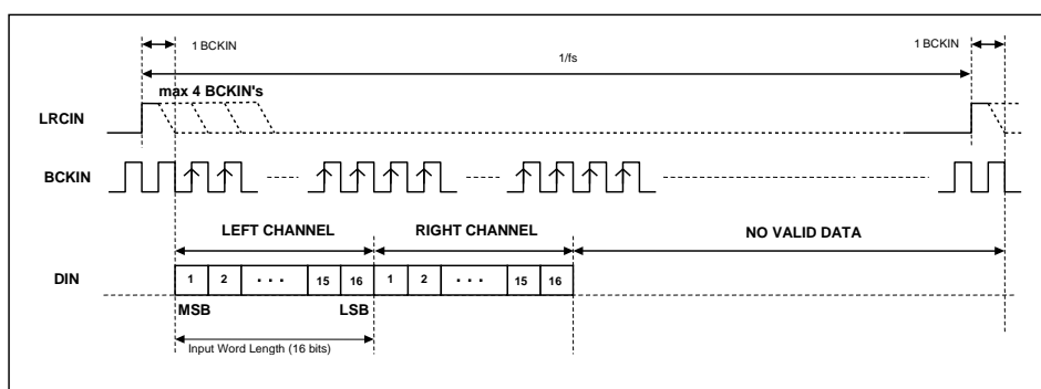
Figure 9 DSP 'Early' Mode Timing
