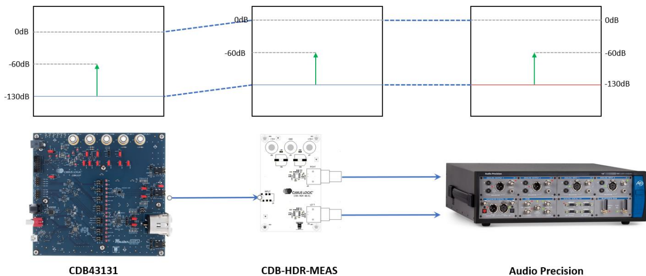
Figure 17 Testing With CDB-HDR-MEAS
