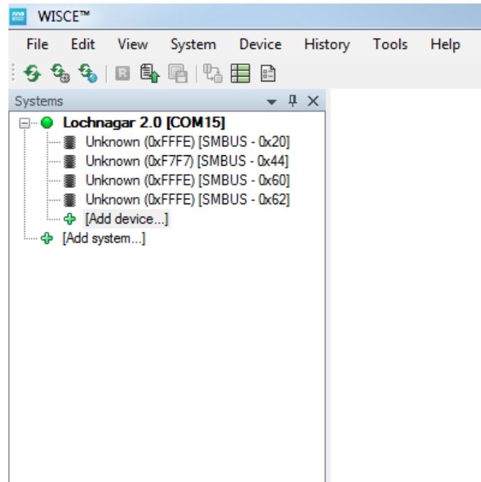
Figure 19 Found Devices
