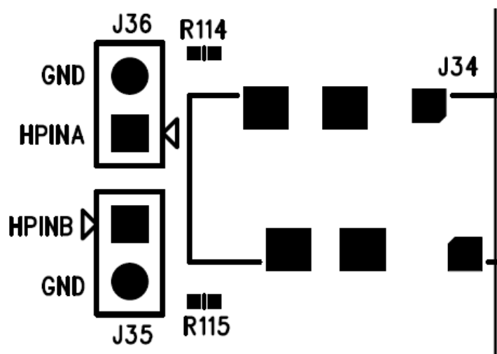
Figure 9 1/8" Headphone Jack and APx connectors for QFN
