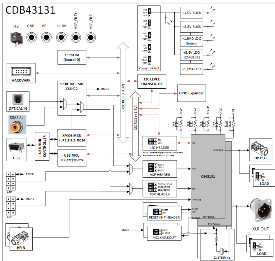
Figure 1 CDB43131 Board Block Diagram
