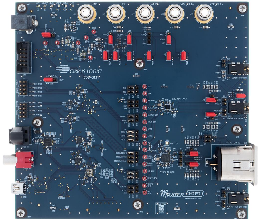
Figure 2 CDB43131 Base Board
