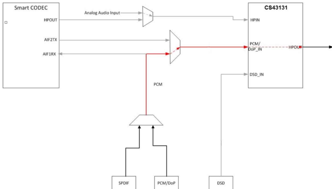
Figure 44 PCM Playback Data Flow
