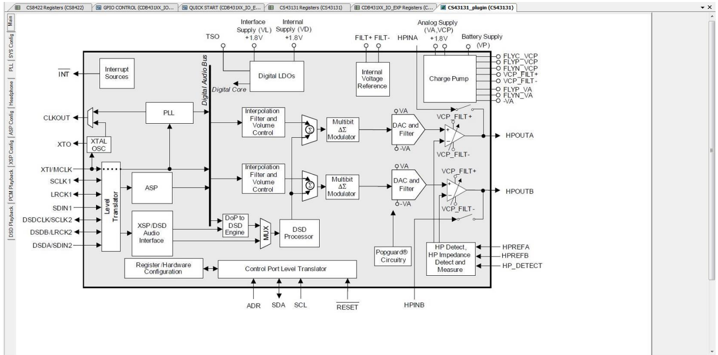
Figure 26 CS43131 Plugin
