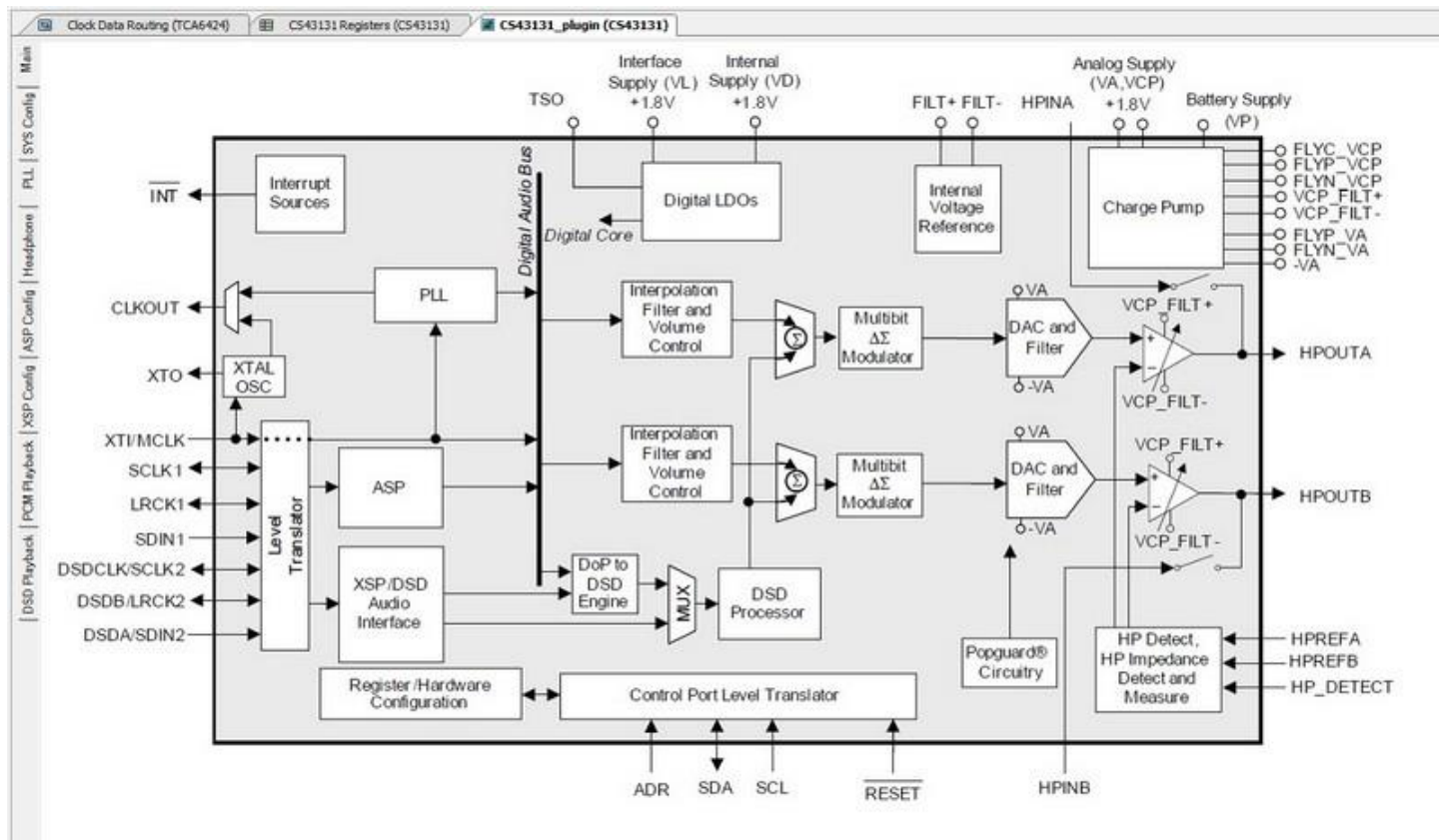
Figure 28 Main tab
