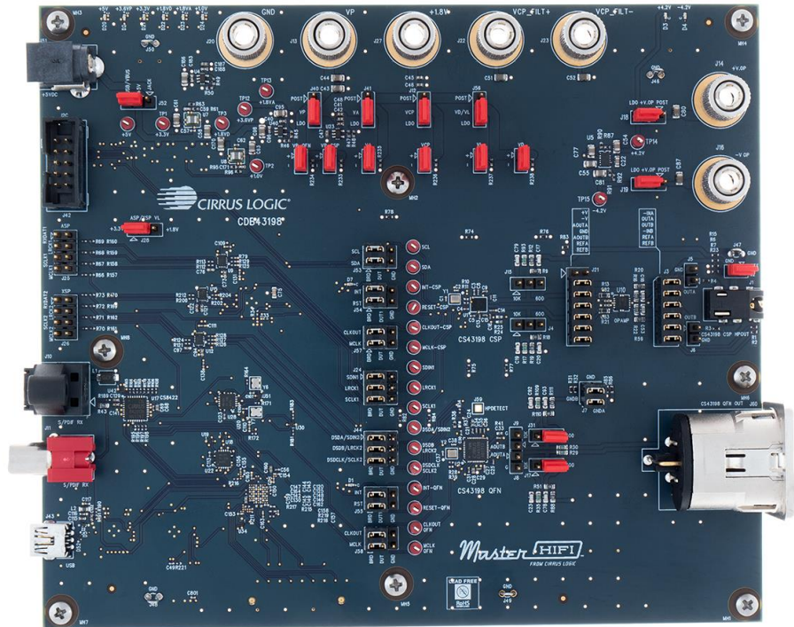
Figure 2 CDB43198 Base Board
